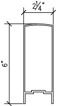
2 1/4" x 6" DOMED TOP CAP
