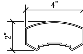
4" x 2" TOP CAP
