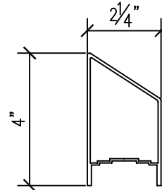
2 1/4" x 4" SLANTED TOP CAP
