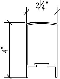
2 1/4" x 4" DOMED TOP CAP
