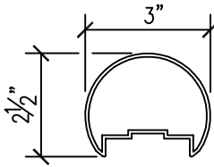
3" ROUND TOP CAP
