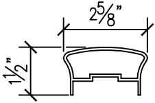
2 5/8" x 1 1/2" TOP CAP
